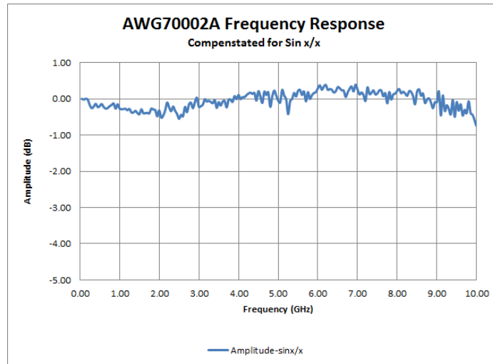
AWG70002A frequency response at 25 GS/s with \text{Sin}(x)/x response mathematically removed from measured data
