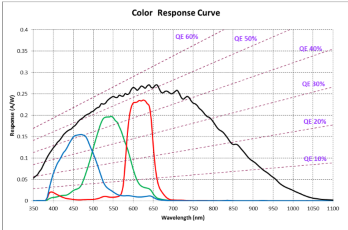
Spectral response curve for Miro N5
