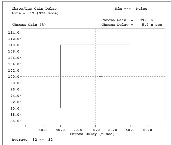
Chrominance to Luminance Gain and Delay measurement.
