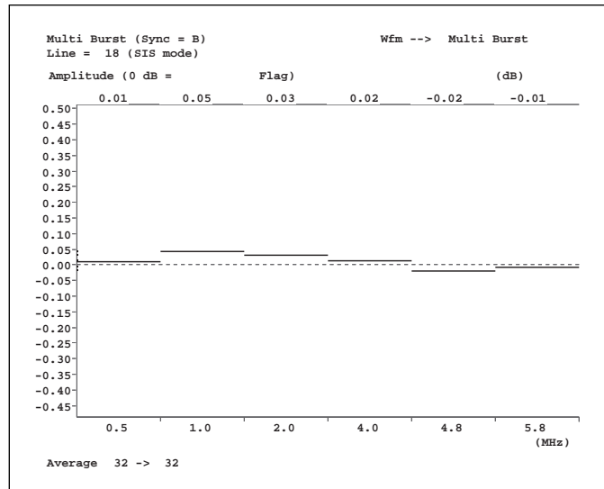
Multiburst measurement.
