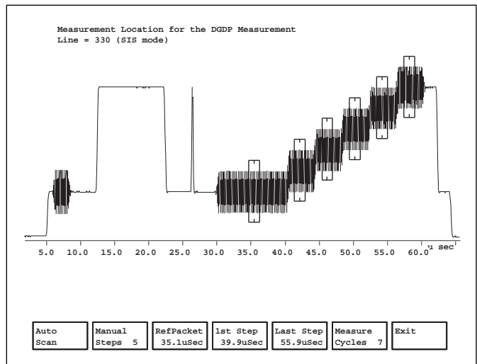
Measure Mode DGDP special position acquisition feature.
