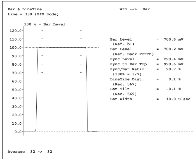
Bar Line Time measurement.
