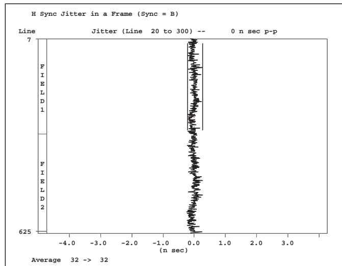
H_Jitter.
